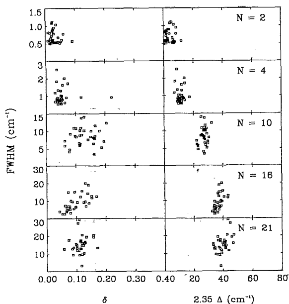
FIG. 2. Left-hand side: Correlation between the FWHM of the subspectra and the Ar-Ar rms bond fluctuation of the associated trajectory. Right-hand side: Correlation between the FWHM of the subspectra and the static approximation for the spectral width.
