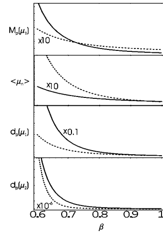
FIG. 2. Top panel: the p th moment of the photon arrival times distribution M_p(\mu_n) vs \beta for n=1 (solid line) and p=2 (dashed line). Second panel: the ensemble-averaged n th moment of photon arrival times \langle \mu_n \rangle for n=2 (dashed line) and for n=1 (solid line). Third panel: the difference d_p(\mu_n) of the p th moment of the photon delay times distribution M_p(\mu_n) and the ensemble average of the n th moment of photon delay times \langle \mu_n \rangle taken to p th power vs \beta for p=3, n=1 (dashed line) and for p=2, n=1 (solid line). Bottom panel: the difference d_p(\mu_n) vs \beta for p=3, n=2 (dashed line) and M_p(\mu_n) for p=2, n=2 (solid line). For clarity some curves were multiplied by the factors as indicated, \sigma = a = 1 .
