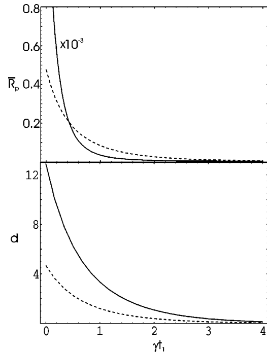
FIG. 3. Top panel: the reduced ratio \bar{R}_p(t_1) = R_p(C_{nm}, \gamma t_1) - r_p(\mu_n)r_p(\mu_m) vs \gamma t_1 for n=m=1 , \beta=1 ; p=2 [ \bar{R}_p(t_1) , dashed line] and p=3 [ 10^{-3}\bar{R}_p(t_1) , solid line]. Bottom panel: difference d(t_1) = \langle \tau^n(0) \tau^m(\gamma t_1) \rangle - \langle \mu_n \rangle \langle \mu_m \rangle vs \gamma t_1 for n=m=1 ; \beta=1 (dashed line) and \beta=0.8 (solid line); a=\sigma=1 .
