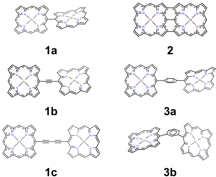
FIG. 1. Various Zn-Ni porphyrin dimers in this study
