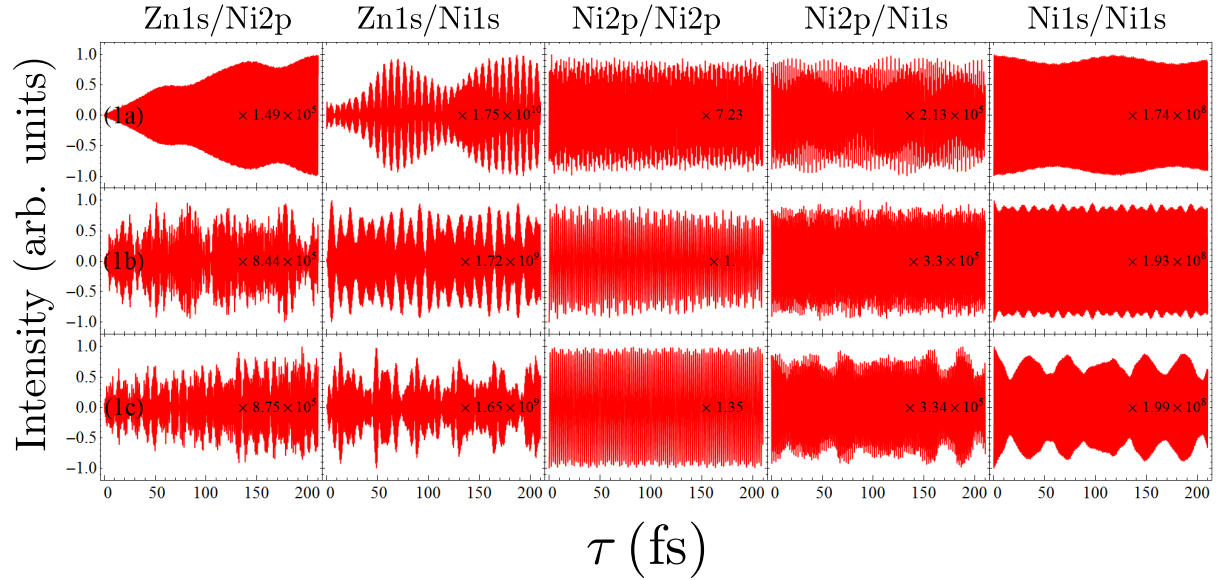
FIG. 4. Comparison of the I2P-SXRS signals for dimers 1a, 1b, and 1c, for five different combinations of pump and probe.
