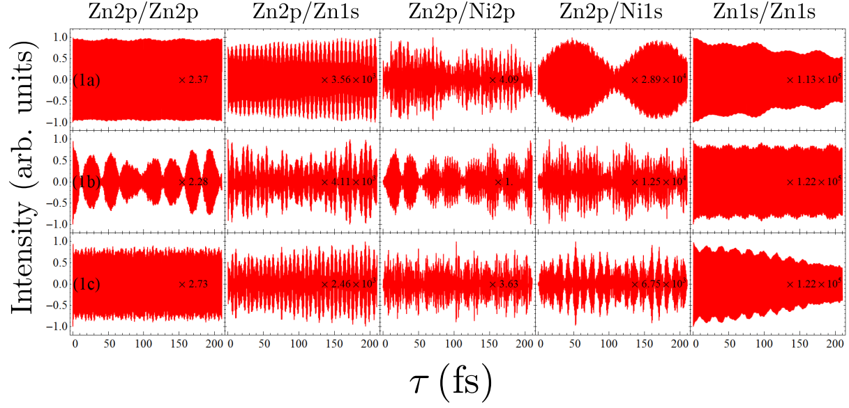
FIG. 3. Comparison of the I2P-SXRS signals for dimers 1a, 1b, and 1c, for five combinations of pump and probe. All signals have been normalized to lie between -1 and 1 prior to plotting. The relative scale is indicated as a multiplier on each signal, i.e. the largest signal, the Zn2p/Ni2p for dimer 1b, has a multiplier of 1.
