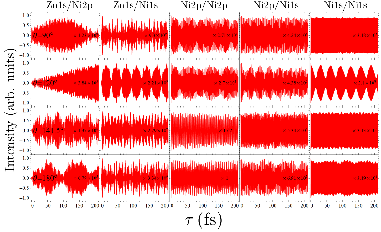
FIG. 11. Comparison of the I2P-SXRS signals for dimer 1b with four different intermonomer angles, for five different combinations of pump and probe.
