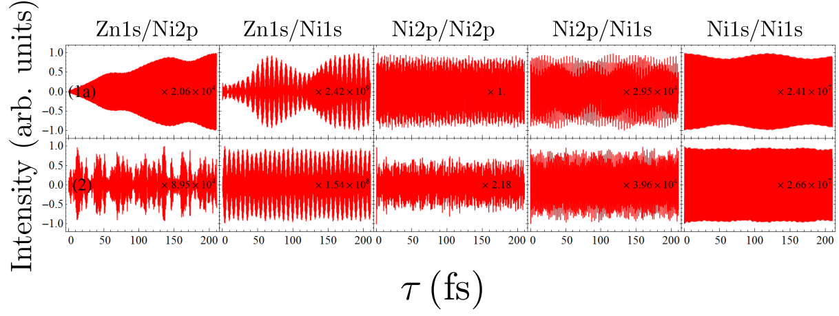
FIG. 7. Comparison of the I2P-SXRS signals for dimers 1a and 2, for five different combinations of pump and probe.
