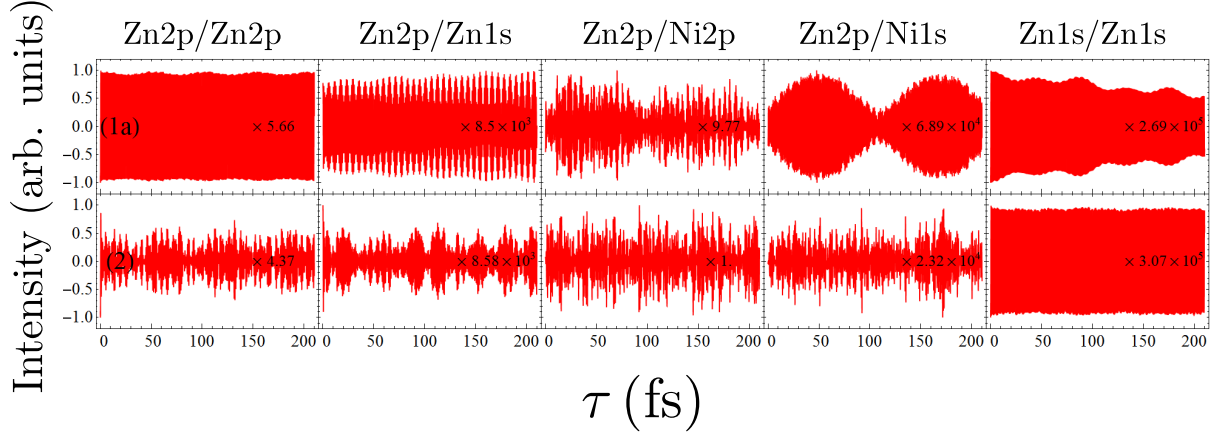
FIG. 6. Comparison of the I2P-SXRS signals for dimers 1a and 2, for five combinations of pump and probe.
