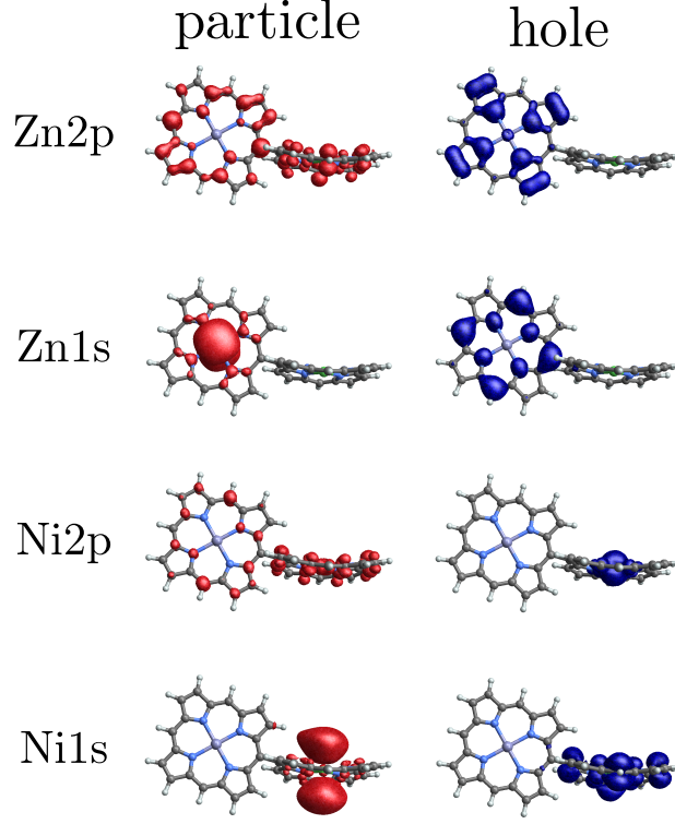
FIG. 5. Electron and hole densities for window wavepackets prepared using the four pulses considered here, for dimer 1a. The zinc monomer, which is planar, is on the left and the nonplanar nickel monomer is on the right. Particle and hole isosurfaces are shown in red and blue, respectively. The wavepackets were normalized prior to plotting.
