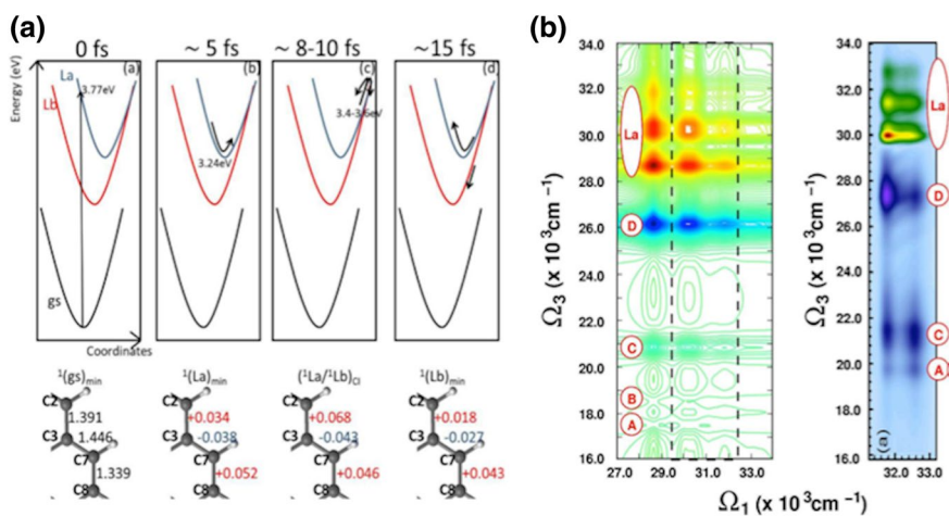
Fig. 15 a Schematic representation of the photophysics of pyrene based on quantum-classical dynamics. The dominant bond deformations are given, with the GS equilibrium geometry used as a reference. b Theoretical (left panel) and experimental (right panel) quasi-absorptive 2D electronic spectra of pyrene for a delay time t_2 in the picosecond range ( t_2 = 1 ps in the experiment) obtained through pumping at the frequency of the L_a transition and supercontinuum probing in the UV–Vis region. Color code: GSB (red), ESA (blue). Note that the color code is inverted with respect to other figures so as to enable easy comparison with the experimentally reported spectrum. Reproduced from data reported in Ref. [93]
