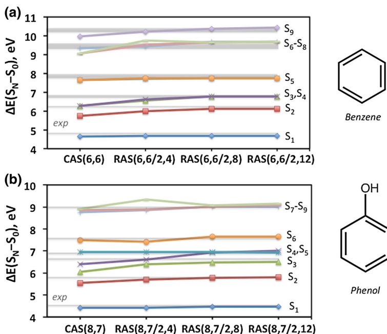
Fig. 4 CASSCF//PT2 and RASSCF//PT2 vertical S_0 \rightarrow S_N excitation energies (in eV) of benzene and phenol monomers in a vacuum obtained using the large ANO-L(432,21)-aug basis set at different levels of theory. Minimal active space CAS(X,Y) results are compared to restricted active space (RAS2/RAS3) calculations with an increasing number of virtual orbitals (4, 8 and 12) and experimental values (gray bars, indicating ranges of experimental absorption maxima recorded). Reproduced from data reported in Ref. [58]
