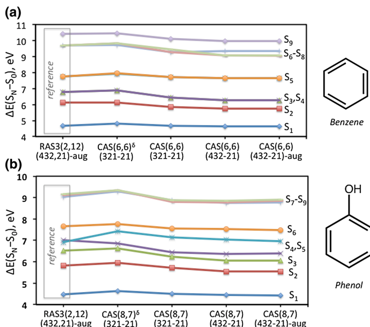
Fig. 8 CASSCF/PT2 and RASSCF/PT2 vertical S_0 \rightarrow S_N excitation energies (in eV) of benzene and phenol monomers in a vacuum obtained at various levels of theory. Reference data are those computed at the RAS3(2,12)/PT2/ANO-L(432,21)-aug levels and are compared to cheaper computational approaches, including minimal (full-valence) active spaces ( mAS ), i.e. CAS(6,6) and CAS(8,7) for benzene and phenol, respectively, with various ANO-L basis sets and refined mAS ( r-mAS ) δ with the smallest ANO-L(321-21) basis set. Reproduced from data reported in Ref. [58]
