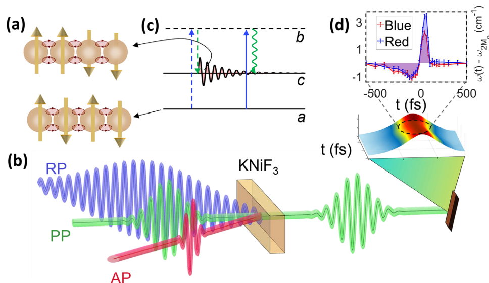
Figure 1. Sketch of the time-resolved FSRS experimental scheme for probing magnon dynamics in KNiF 3 . a,b) Two-magnon excitations are coherently stimulated by the joint action of a picosecond RP and a broadband femtosecond PP, that generates two spin flip events occurring on neighboring sites. A further interaction with the RP followed by a final free induction decay enables to probe the excited magnons as Raman gain or Raman loss. In panel c), we report the energy ladder diagram representing the SRS interaction in the red side, where a indicates the ground state, b represents a virtual electronic level, while c is a two magnon excited state. The presence of an AP pulse triggers the dynamics of interest and, at the same time, modifies the Raman spectrum due to cross-phase modulation with the RP. d) By varying the time delay between AP and RP–PP pair, the photoinduced modification of the 2ML peak position can be monitored. All the pulses are tuned off-resonant with the sample absorption, ensuring that electrons are not excited upon photo-irradiation.
