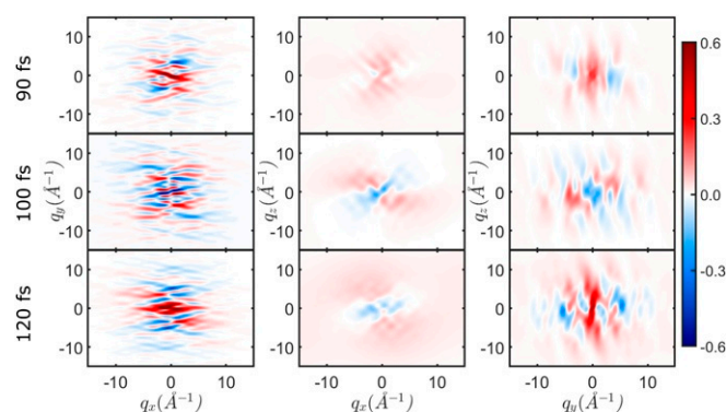
Fig. 5. Two-dimensional diffraction patterns of the coherence contribution (v in Eq. 3) in the q_{xy} , q_{xz} , and q_{yz} planes, while integrating over the respective other direction. The signal emerges at 90 fs, where a vibronic coherence builds up due to the Coln passage. Phase changes between positive (red) and negative (blue) contributions can be observed in all three planes. The complete movie is provided as electronic supplement (Movie S4).
