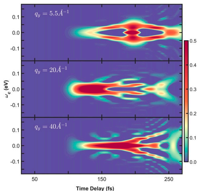
Fig. 7. Wigner representation (Eq. 8) of the coherence diffraction image in Fig. 6. For the spectrogram in Top , a temporal slice was taken from term (v) in Fig. 6 at 5.5 \text{ \AA}^{-1} momentum transfer. The spectrograms in Middle and Bottom were calculated from temporal traces at 20 and 40 \text{ \AA}^{-1} accordingly.
