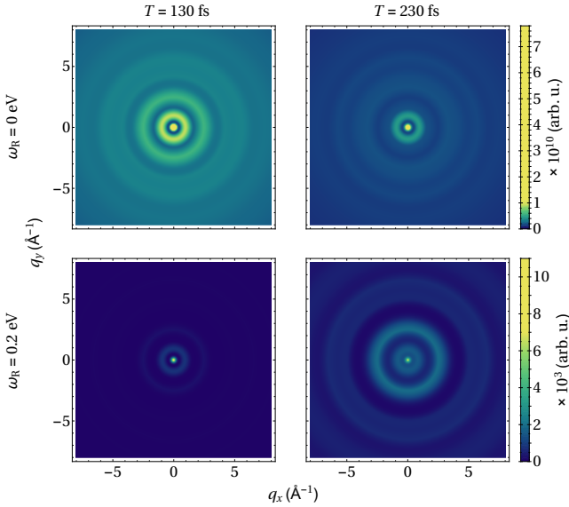
Figure S1. Time- and frequency-resolved CUPXD of azobenzene molecules. The signal is shown at the indicated time delays T and Raman frequencies \omega_R . The q dependence of the inelastic signal at \omega_R = 0.2 eV provides direct access to the temporal and spatial dependence of the coherences during the passage of the molecular wavepacket through a conical intersection.
