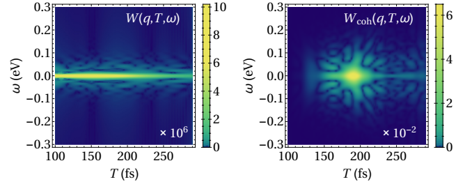
Figure S2. Wigner spectrogram. The spectrograms W(q, T, \omega) and W_{\text{coh}}(q, T, \omega) [Eq. (S1)], for the total signal S(q, T) in Eq. (S2) or for the part stemming exclusively from the coherences, are shown in arbitrary units for a representative momentum transfer of q = 3.3 \text{   }^{-1} , assuming a coherent X-ray pulse of duration \tau = 3 fs and centered at variable time delay T . The spectrogram at large frequencies \omega highlights the coherence contribution. However, in contrast to the frequency-resolved signals discussed in the main text, the frequency information is here extracted from the temporal features of the signal. In an analysis based on Wigner spectrograms, both temporal and spectral information depend on the precise determination of the pulse central time T , whereas temporal and spectral information are independently measured in covariance X-ray diffraction.
