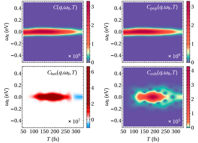
Fig. 3. Temporally and spectrally resolved CUPXD signal in azobenzene. The signal C(q, \omega_R, T) (Eq. 5) and its three components, C_{\text{pop}}(q, \omega_R, T) , C_{\text{het}}(q, \omega_R, T) , and C_{\text{coh}}(q, \omega_R, T) , are displayed in arbitrary units for q = 3.3 \text{ \AA}^{-1} and \tau = 22 fs as a function of time delay T and Raman frequency \omega_R . Elastic scattering off quasi-stationary populations dominates the narrow spectral region around \omega_R = 0 eV. At higher Raman frequencies, due to the drop in C_{\text{pop}}(q, \omega_R, T) , the inelastic signal allows access to the coherence dynamics with significantly reduced background.
