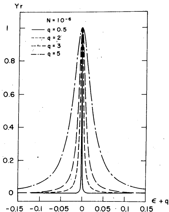
FIG. 5. Dependence of \gamma_r(\epsilon) for predissociation where the internal continuum carries oscillator strengths near the interference dip. The different curves refer to various q values (0.5, 2, 3, 5).
