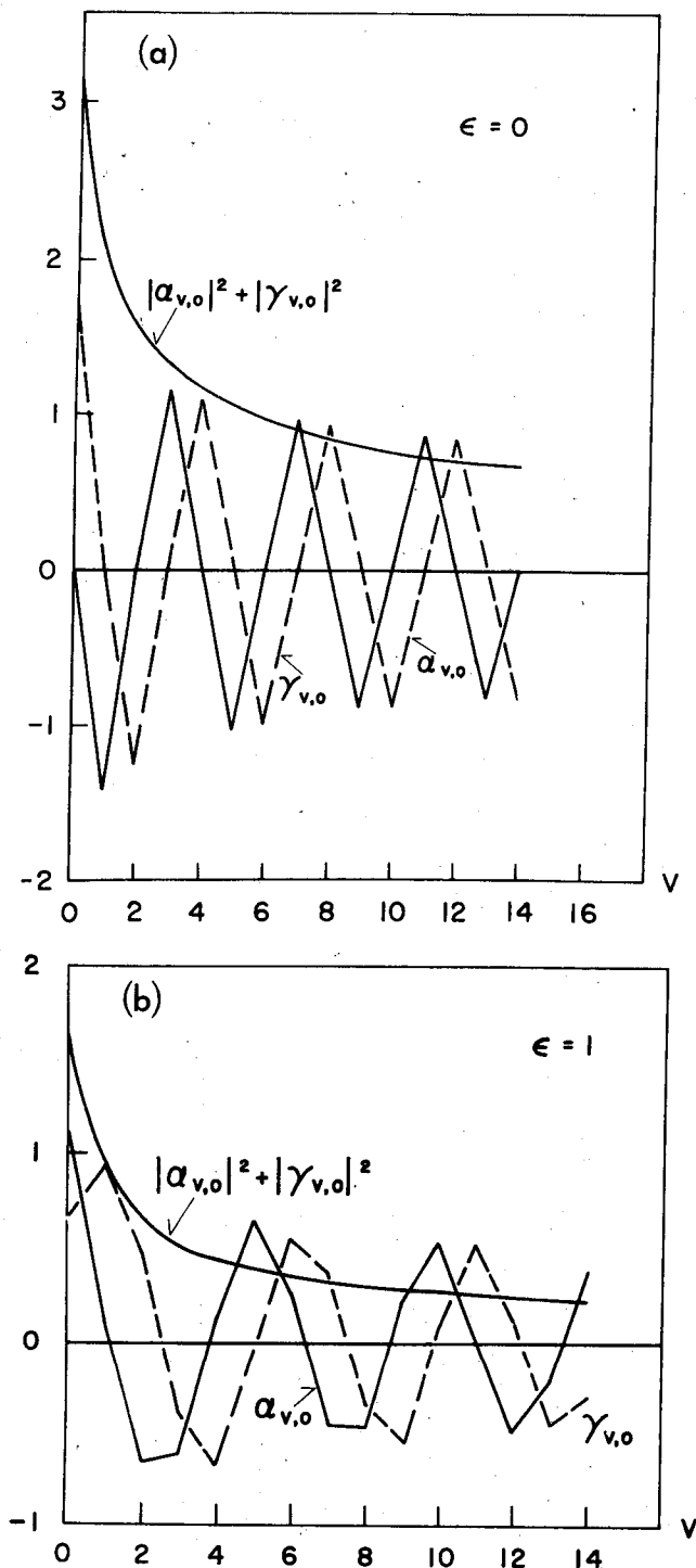
FIG. 2. Raman scattering cross sections from a dissociative continuum characterized by a Gaussian absorption line shape. Plots of the relative populations of the final |g_v\rangle molecular states which are given by
