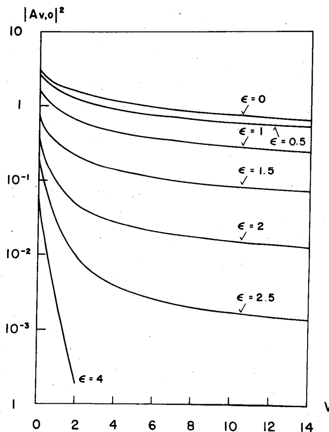
FIG. 3. Plots of the Raman intensities for scattering from a dissociative continuum (see Appendix D). Plots are given for various values of the reduced energy parameter \epsilon .
