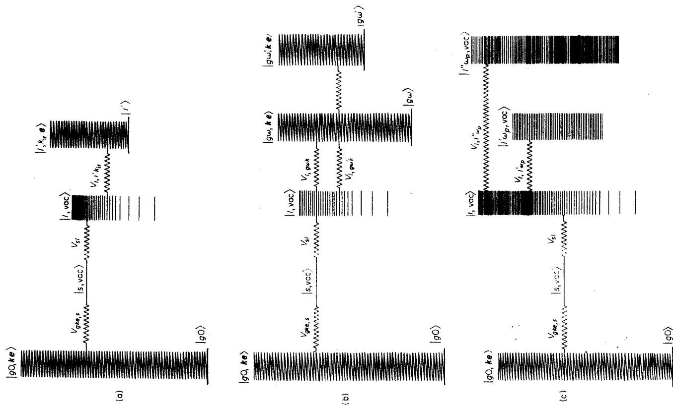
Figure 10.6 Sequential decay schemes. (a) Sequential decay by i.r. emission. (b) Internal conversion. (c) Vibrational relaxation in the intramolecular manifold due to medium perturbation
