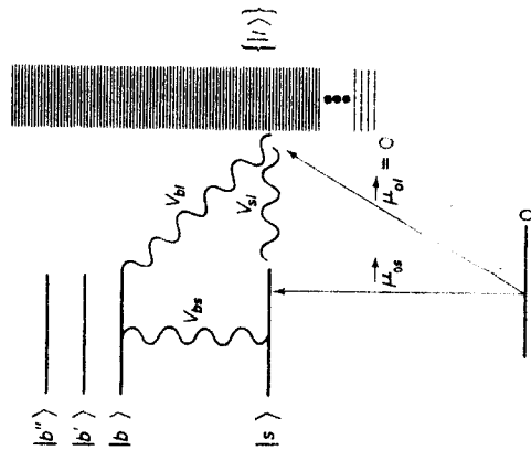
Figure 10.1 A schematic representation of the relevant molecular states and couplings. Wavy lines represent intramolecular coupling. Arrows indicate dipole coupling via the interaction with the radiation field
