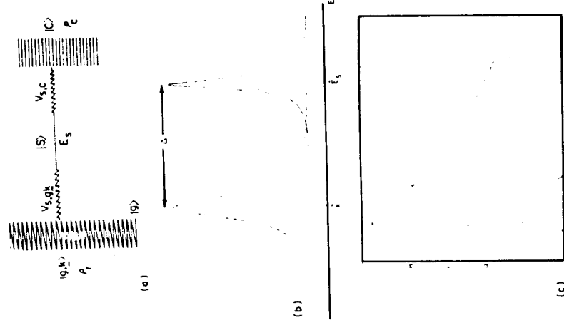
Fig. 2. (a) Energy level scheme for photon scattering from a single isolated resonance. (b) Energy profile for a near resonance photon scattering experiment. (—) L(E) , lineshape of the isolated resonance (a Lorentzian around \bar{E}_s with width \Gamma_s ), (---) |L(E)|^2 , power spectrum of the light pulse around \bar{k} which may assume an arbitrary form. (c) Molecular decay amplitude [C_{ss}(t)] and pulse field amplitude [\varphi(t)] in a time-resolved photon scattering experiment from an isolated resonance. (---) C_{ss}(t) [Eq. (88)], (—) \varphi(t) [Eq. (91)].
