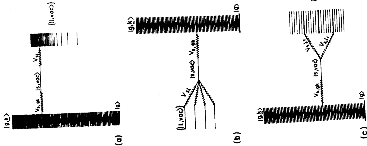
Fig. 1. Basic level schemes for radiative and interstate coupling in polyatomic molecules. (a) A statistical large molecule, (b) a small molecule, and (c) intermediate level structure in a large molecule.
