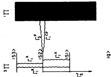
Fig. 5. Energy level scheme for spontaneous and collisionally induced damping processes in I_2 .
