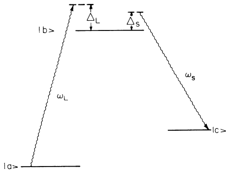
FIG. 1. RRS in the three-level ( |a\rangle, |b\rangle, |c\rangle ) system. The laser and the scattered frequencies are \omega_L and \omega_S , respectively. The corresponding frequency detunings are denoted by \Delta_L and \Delta_S .
