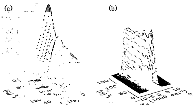
FIG. 3. (a) The three-pulse photon echo signal. (b) The impulsive pump-probe signal.
