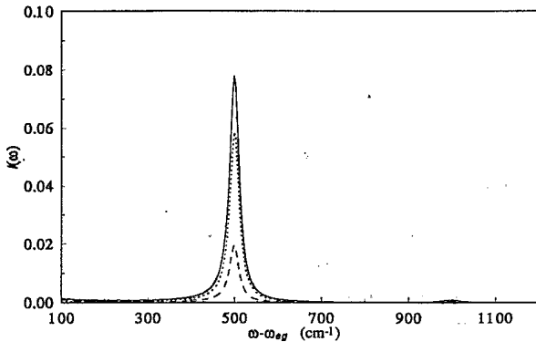
FIG. 4. Absorption spectrum [Eq. (5.19)] with Condon and non-Condon dipole interactions for a weak damping case, \gamma = 0.05\omega_0 . The fundamental 0-0 transition (not shown) is 230 times more intense. The solid line ( \mu' = 0.1, \mu'' = 0.01 ) indicates the non-Condon interaction, whereas the dashed line indicates the Condon approximation. The difference between these two lines is shown by the dotted line.
