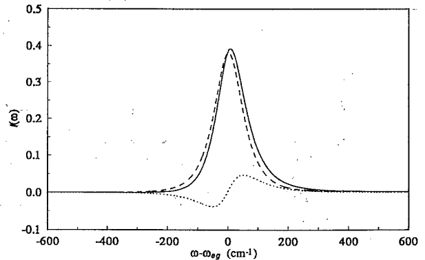
FIG. 5. Absorption spectrum for a strong damping \gamma = 5\omega_0 . Other parameters are the same as in Fig. 4.
