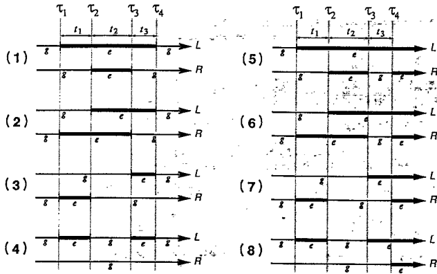
FIG. 3. Doubled-sided Feynman diagrams in fourth order. The paths 1–4 correspond to the process g to g , whereas 5–8 correspond to g to e . The Hermitian conjugate paths of 1–8, which can be obtained by interchanging L and R , respectively, are not shown here.
