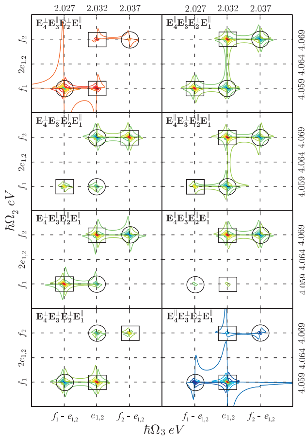
Figure 4 (online colour at: www.pss-b.com ) Chirality effects in the 2D quadrupole correlation spectrum \Im S^{(3)}(t_1 = 0, \Omega_2, \Omega_3) for the cuprous oxide, T = 40 K, n_e = n_r . The sample is oriented in \mathbf{k}_j \parallel [112] direction and we used the notation \mathbf{E}_j^\parallel \parallel [11\bar{1}] , \mathbf{E}_j^\perp \parallel [1\bar{1}0] . The squares mark the absorptive and circles stand for gaining contributions to the response function.
